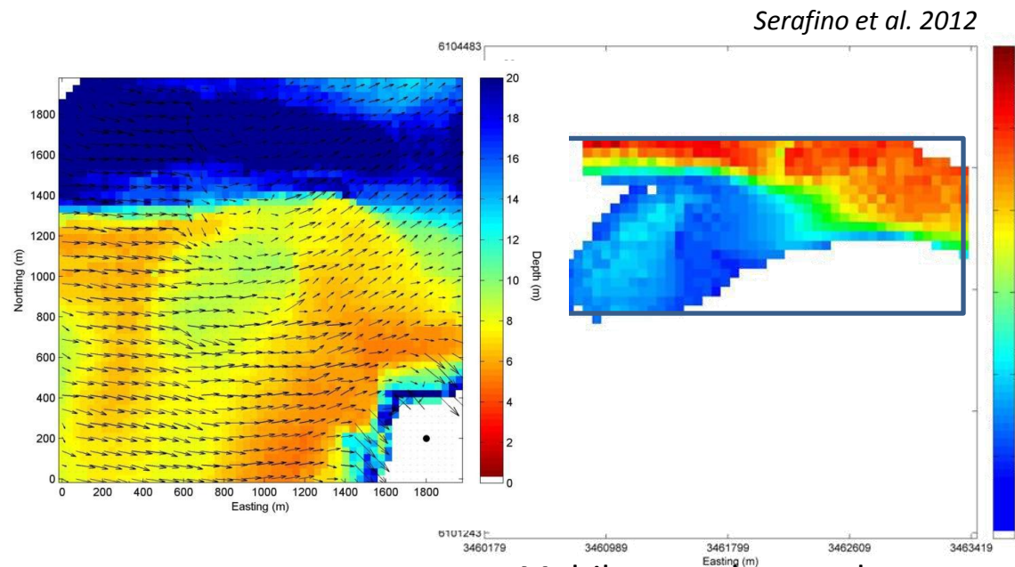
Multibeam echosounder bathymetric data acquisition
